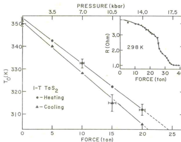
Fig. 1. The variation of T_0 as a function of P . dT_0/dP given in the text was the mean value for both heating and cooling. The insert shows the R -variation with P at 298K. The bars represent the width of the transition and the uncertainty in pressure.
